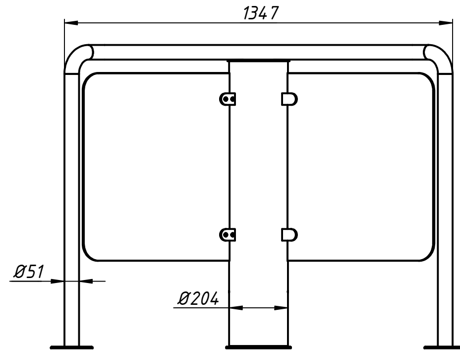
Installation tamplate
