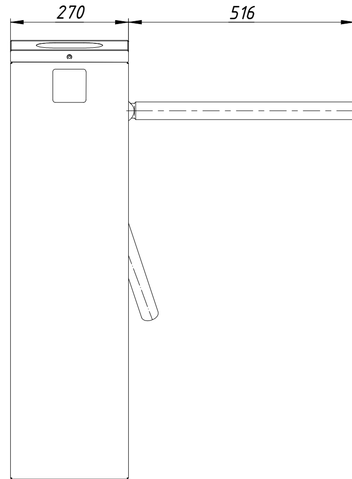
Installation tamplate
