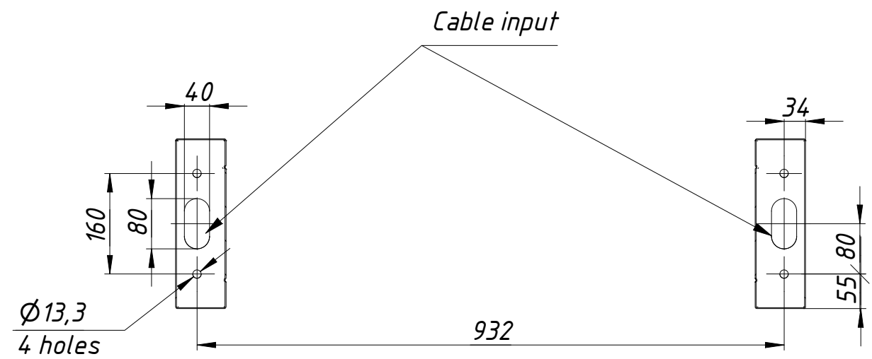
Installation tamplate
